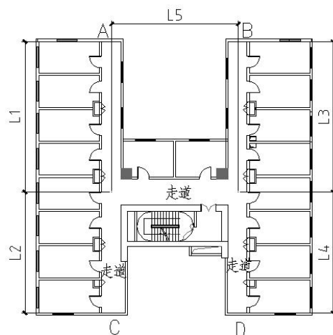
防烟分区长边 L_{\text{长边}} = \max \{ L(A, D), L(B, C), L(A, C), L(B, D), L(A, B), L(C, D) \} 其中 L(A, D) = L1 + L5 + L4 , L(A, C) = L1 + L2 , L(A, B) = L1 + L5 + L3 , 其余类似 附图 12.3.8-3 “H”形走道（一）
